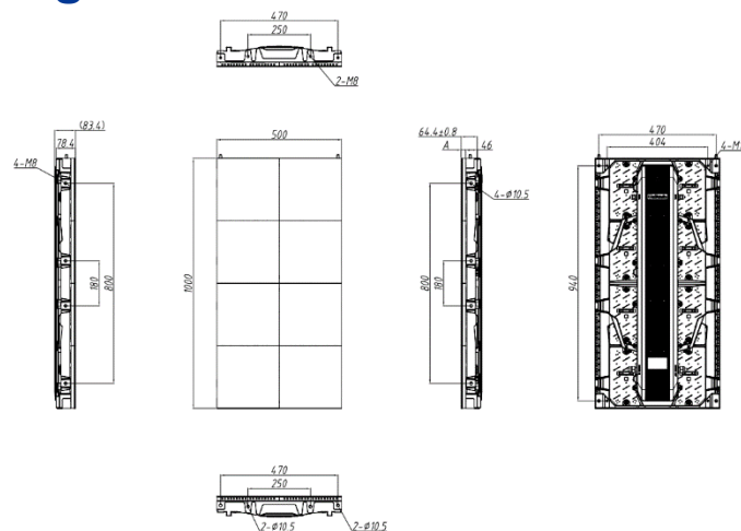
Figure 1 500*1,000mm Drawing of Cabinet
