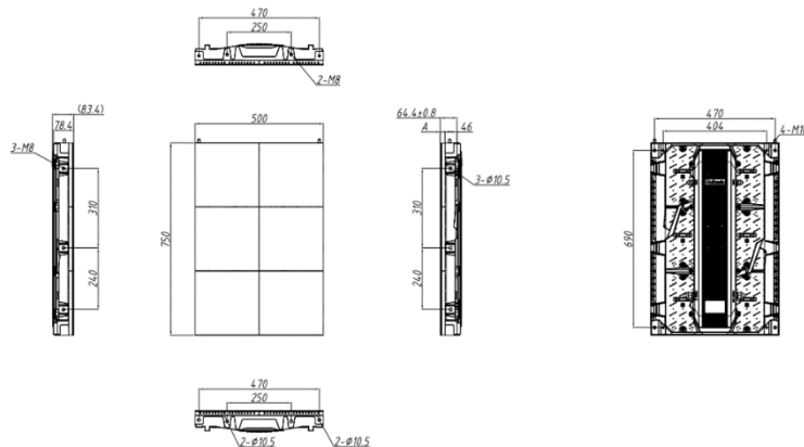
Figure 2 500*750mm Drawing of Cabinet
