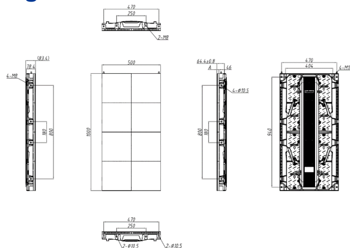
Figure 1 500*1,000mm Drawing of Cabinet
